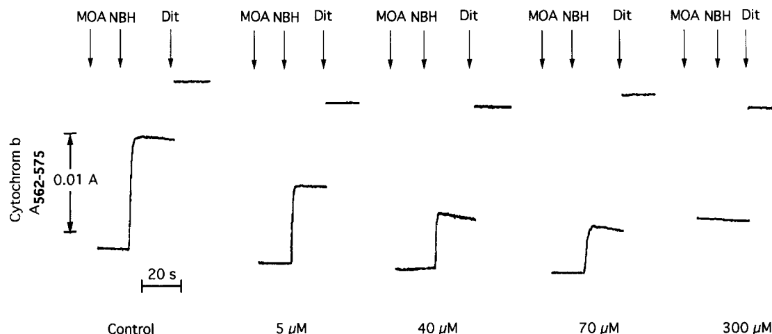
Fig. 3. Inhibition of cytochrome b reduction by preincubation with NOF. Isolated cytochrome bc 1 complex (1.5 \mu M) in incubation medium in the presence of 50 \mu M MOA-stilbene (MOA) was preincubated for 1 min with increasing concentrations of NOF prior to the addition of 15 \mu M NBH. At the end of each experiment the sample was completely reduced by the addition of a few grains of sodium dithionite. The reduction of b cytochromes was monitored at 562 minus 575 nm.
